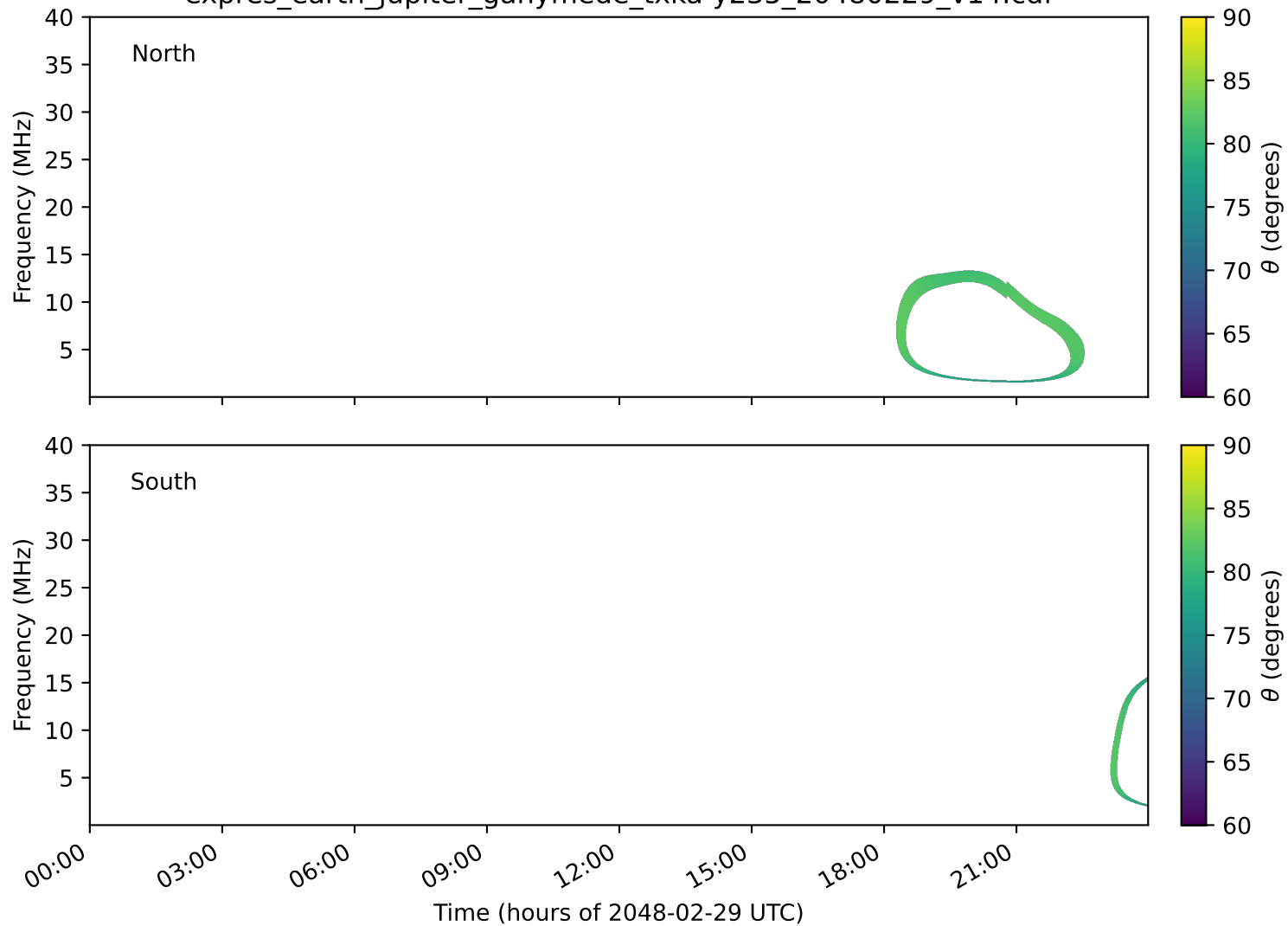
expres_earth_jupiter_ganymede_txka-y235_20480229_v14.cdf
