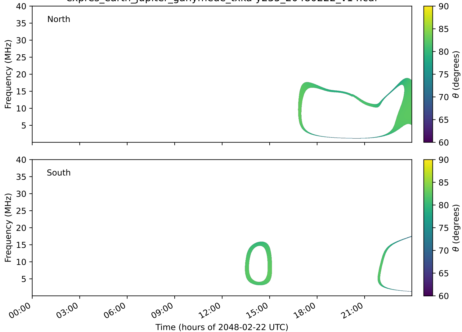
expres_earth_jupiter_ganymede_txka-y235_20480222_v14.cdf
