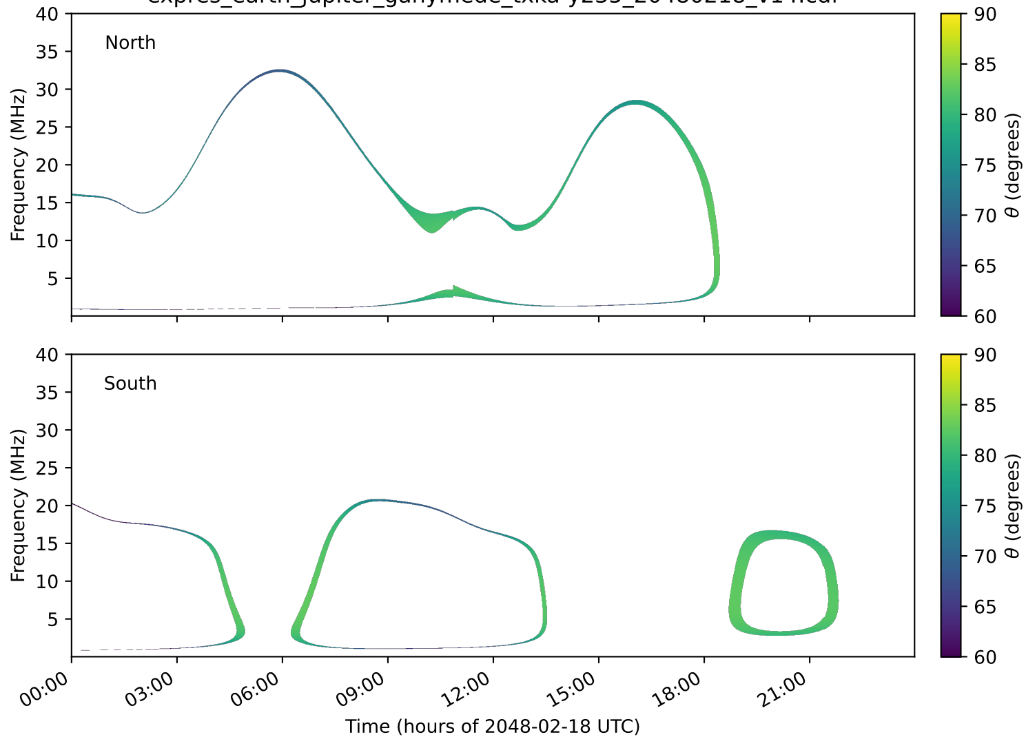
expres_earth_jupiter_ganymede_txka-y235_20480218_v14.cdf
