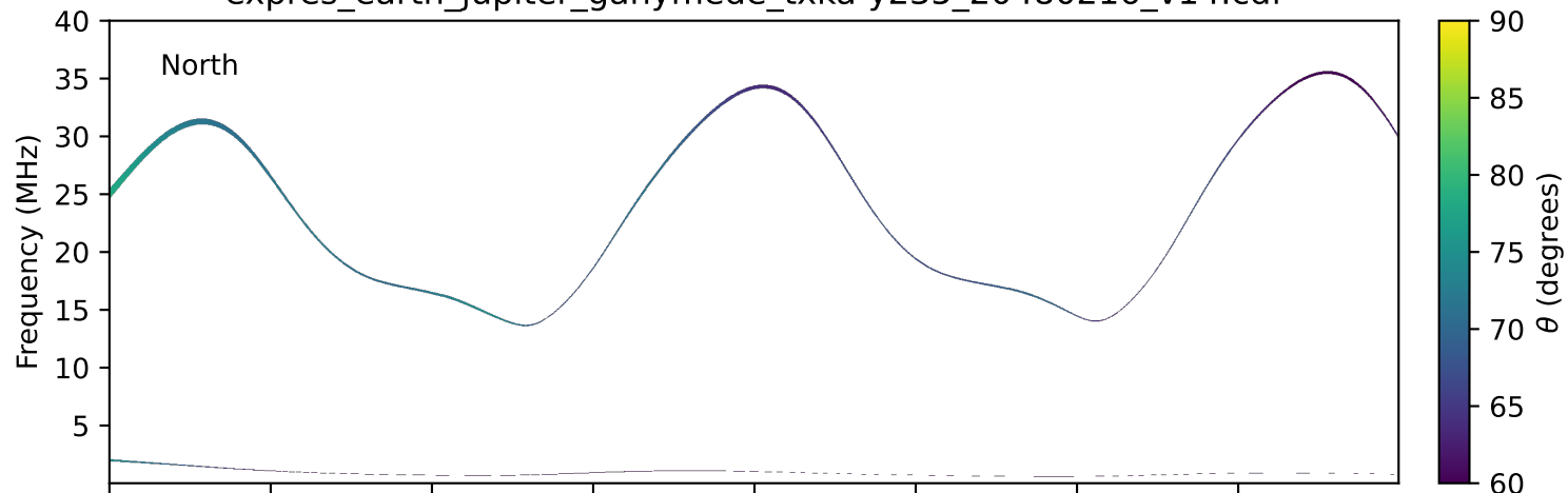
expres_earth_jupiter_ganymede_txka-y235_20480216_v14.cdf
