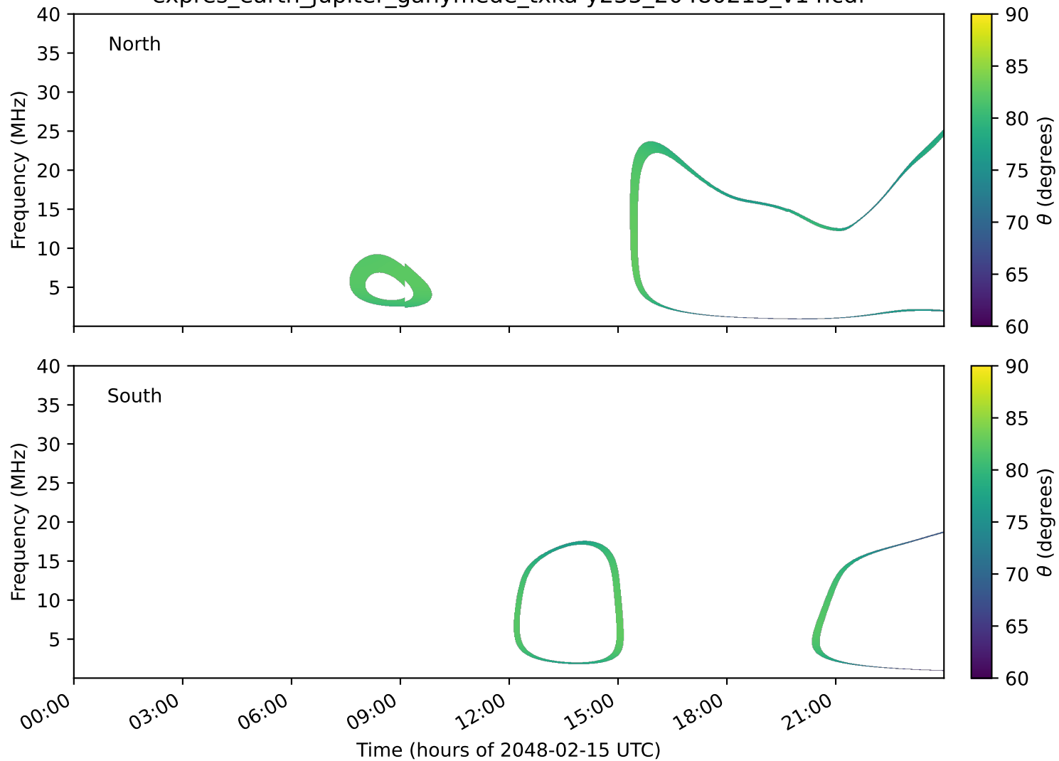
expres_earth_jupiter_ganymede_txka-y235_20480215_v14.cdf
