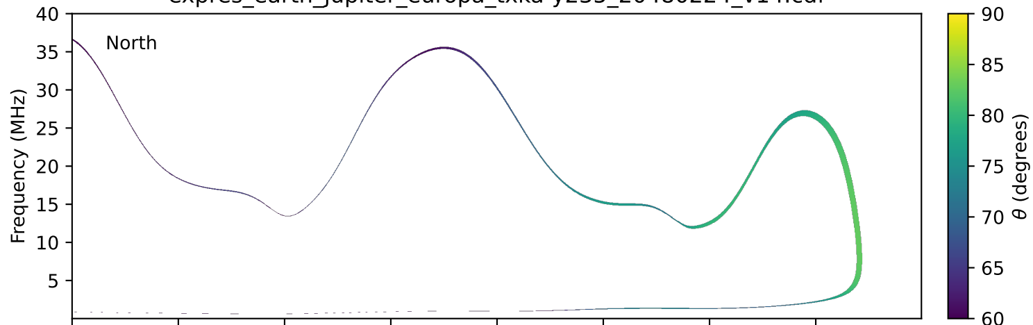
expres_earth_jupiter_europa_txka-y235_20480224_v14.cdf
