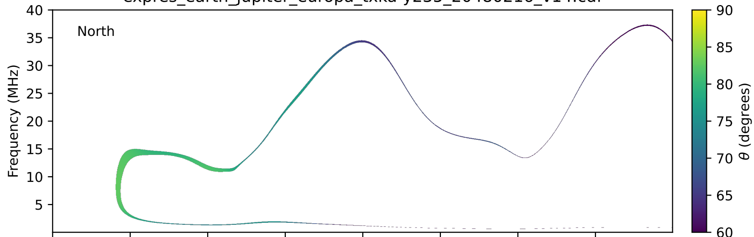
expres_earth_jupiter_europa_txka-y235_20480216_v14.cdf
