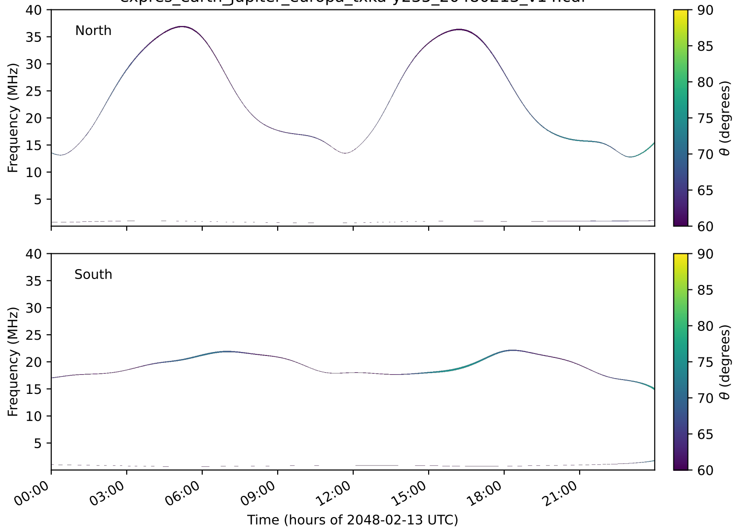
expres_earth_jupiter_europa_txka-y235_20480213_v14.cdf
