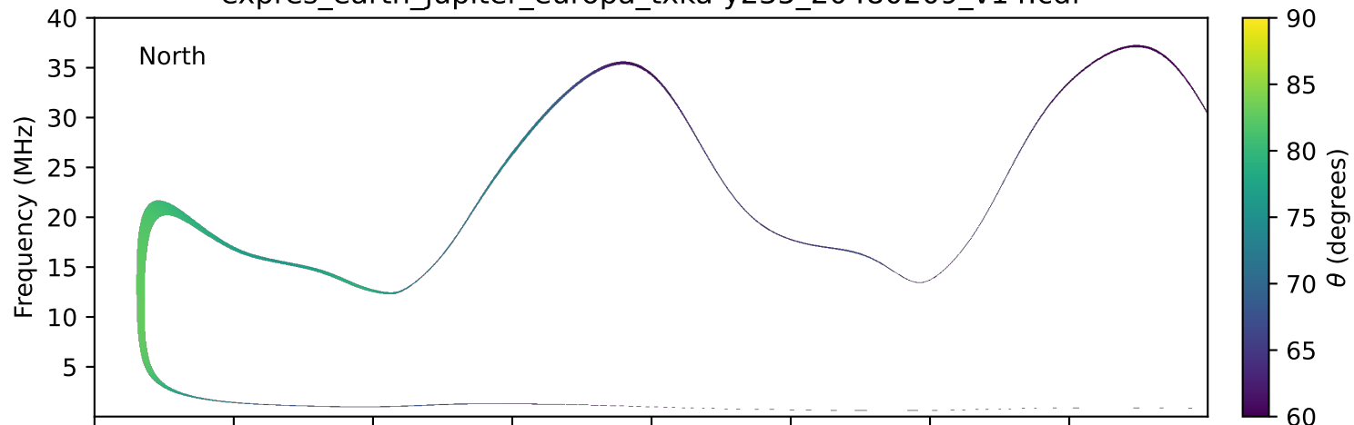
expres_earth_jupiter_europa_txka-y235_20480209_v14.cdf
