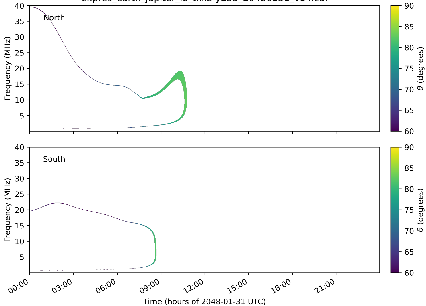
expres_earth_jupiter_io_txka-y235_20480131_v14.cdf
