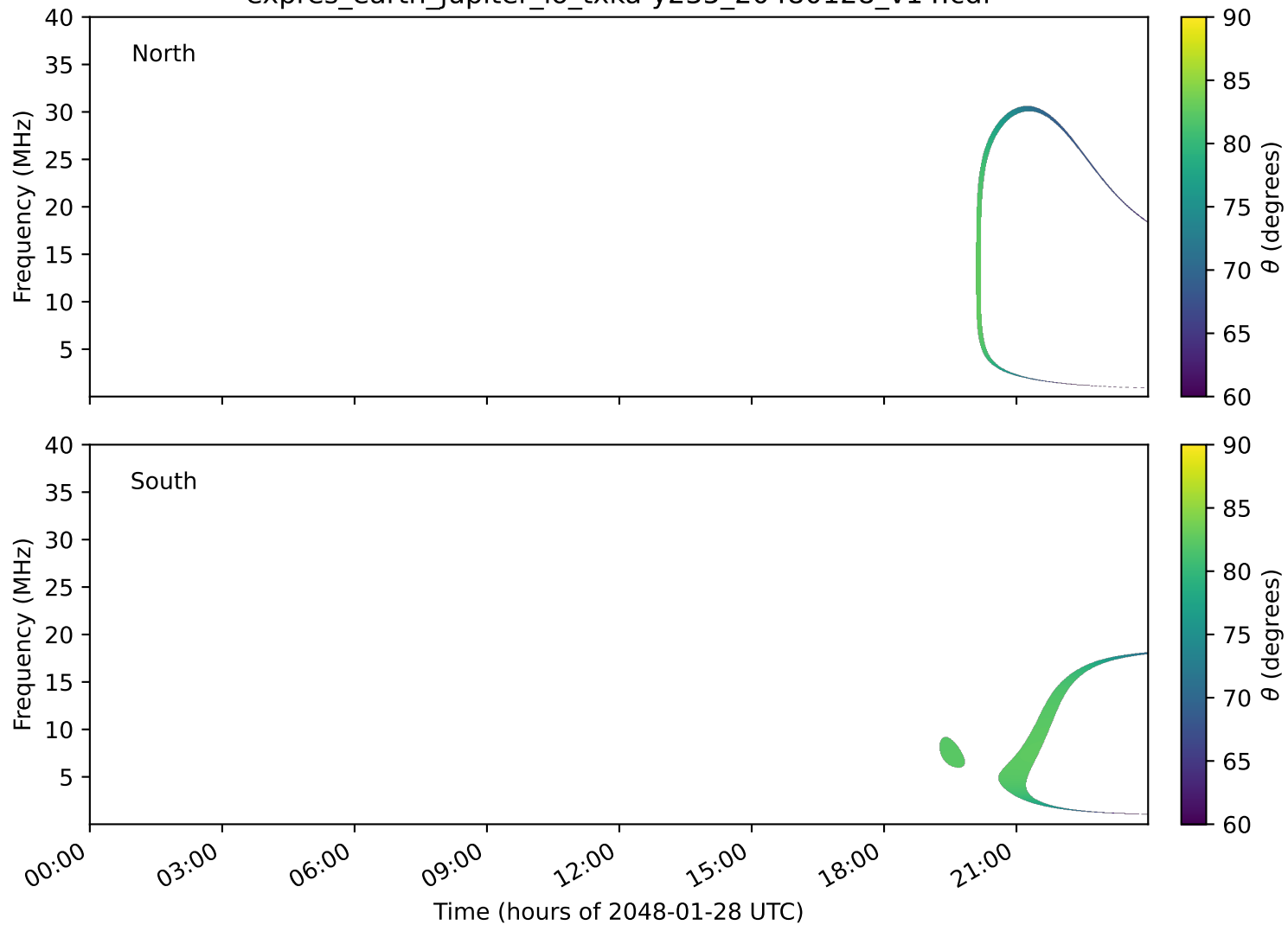
expres_earth_jupiter_io_txka-y235_20480128_v14.cdf
