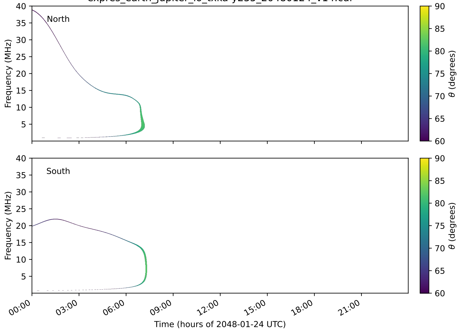
expres_earth_jupiter_io_txka-y235_20480124_v14.cdf
