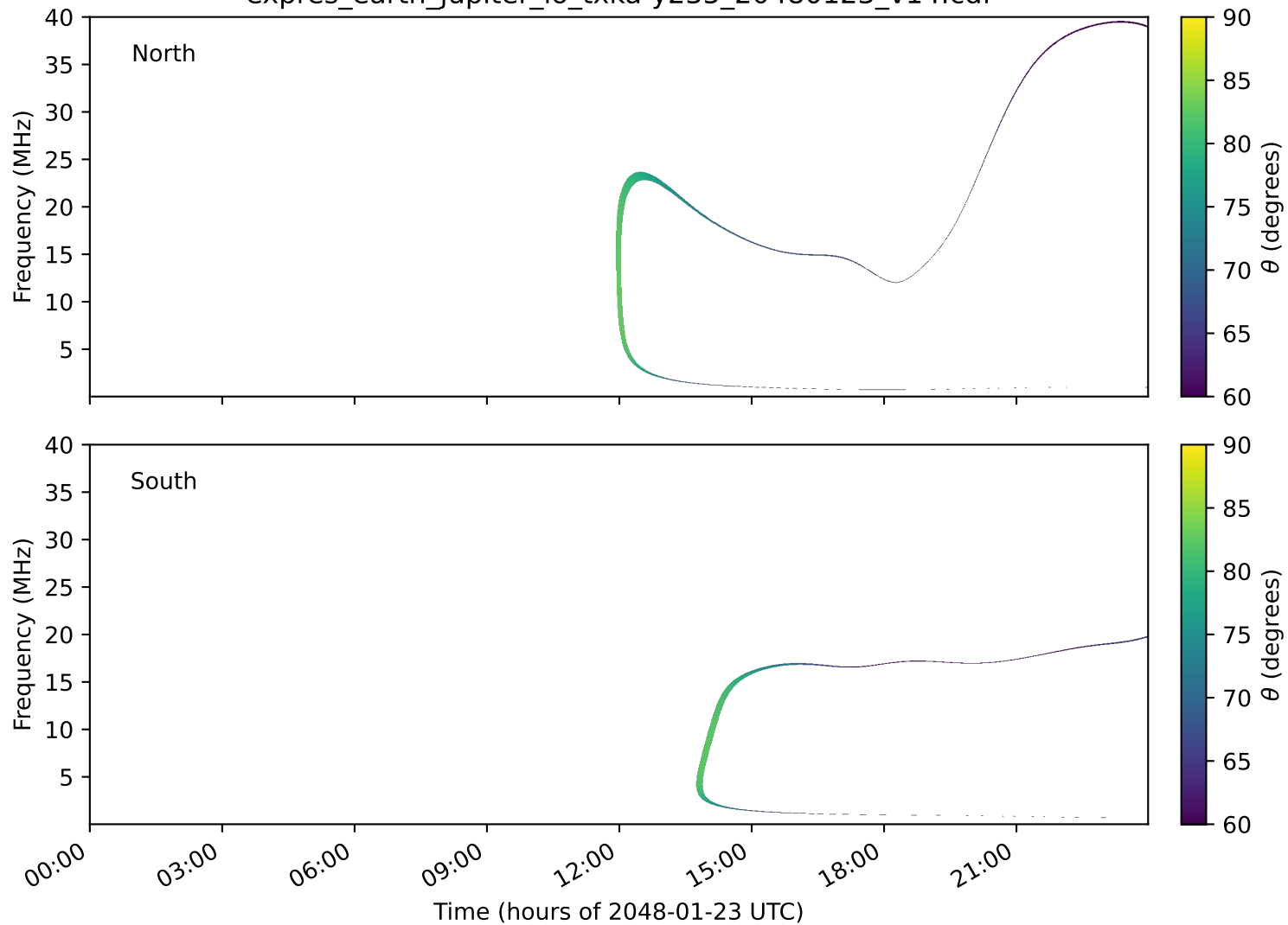
expres_earth_jupiter_io_txka-y235_20480123_v14.cdf
