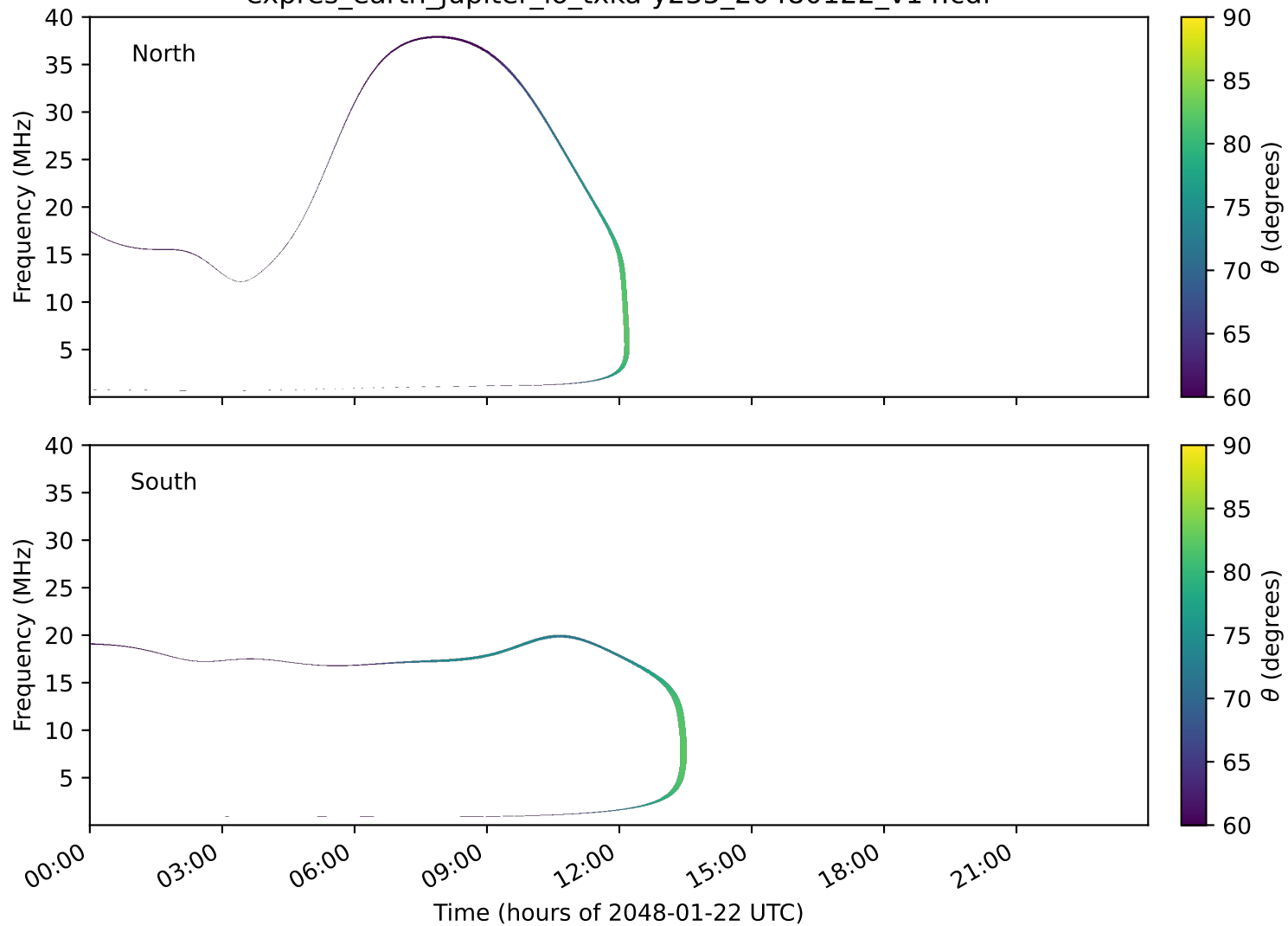
expres_earth_jupiter_io_txka-y235_20480122_v14.cdf
