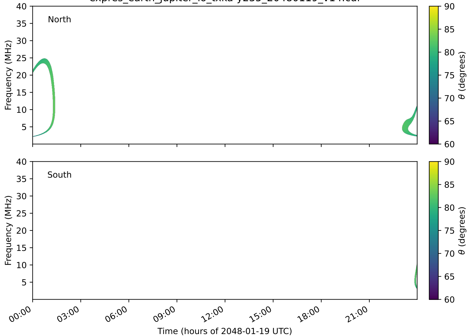
expres_earth_jupiter_io_txka-y235_20480119_v14.cdf
