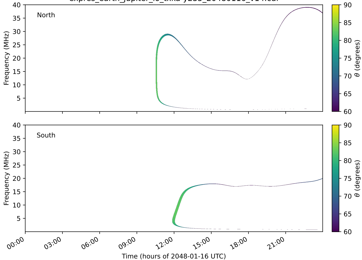
expres_earth_jupiter_io_txka-y235_20480116_v14.cdf
