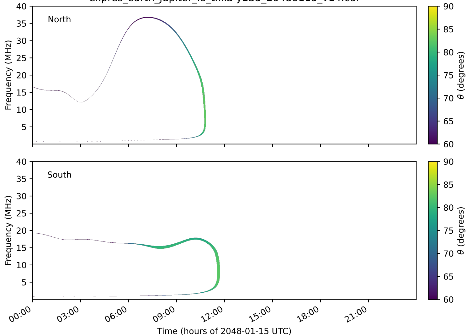
expres_earth_jupiter_io_txka-y235_20480115_v14.cdf
