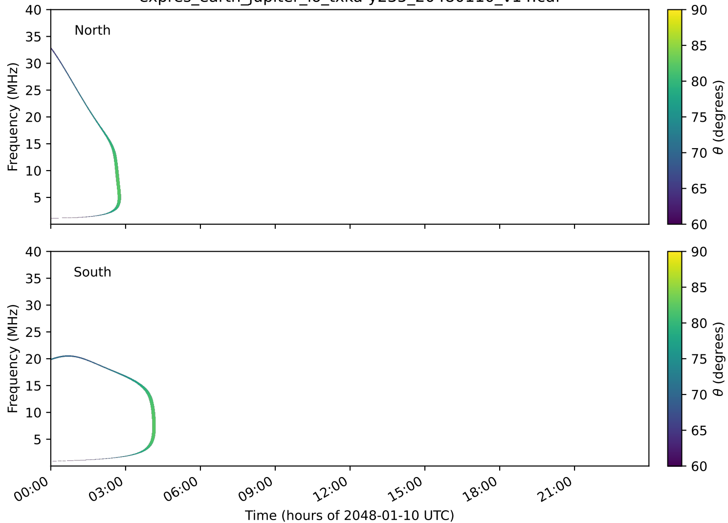
expres_earth_jupiter_io_txka-y235_20480110_v14.cdf
