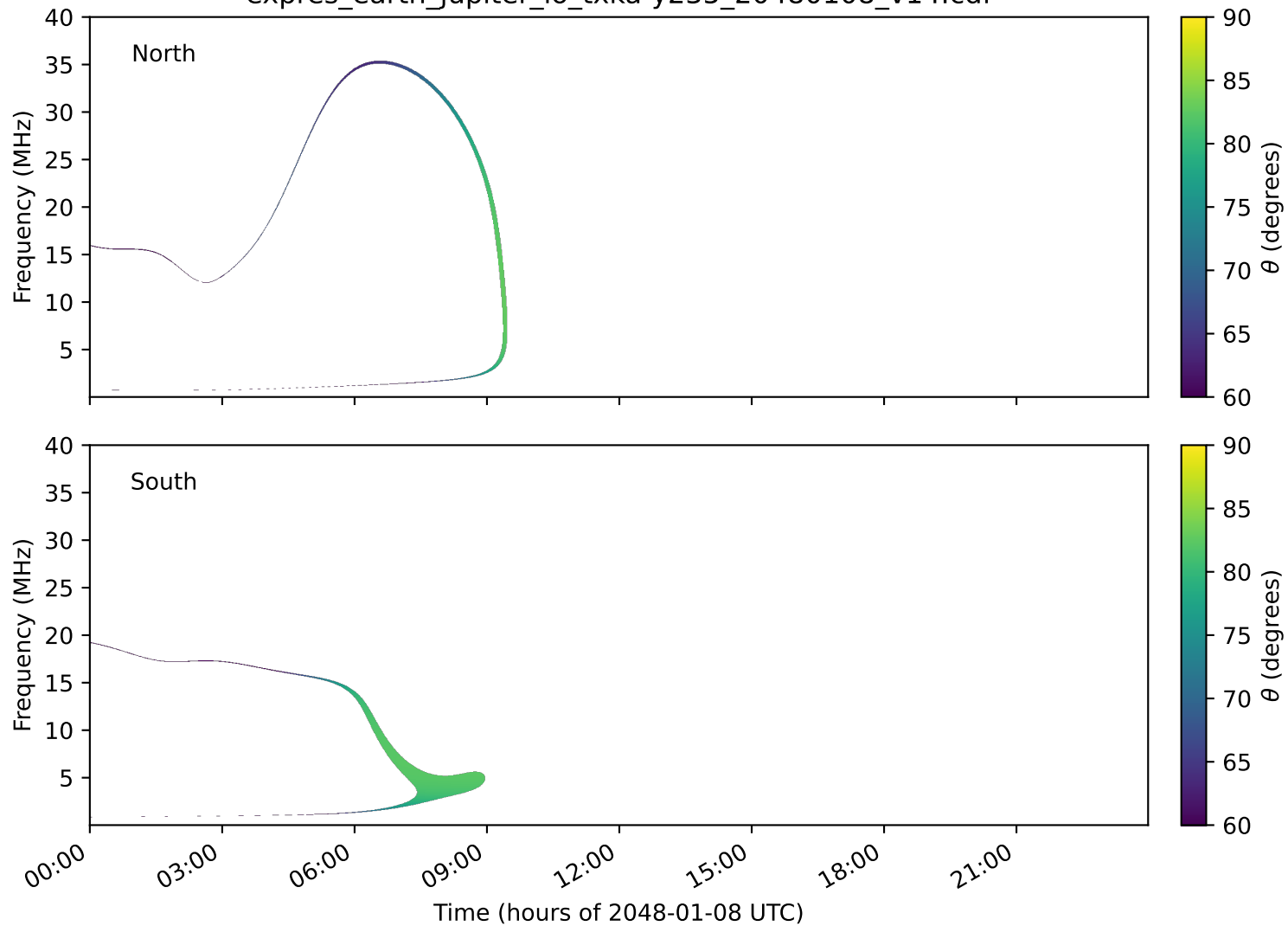
expres_earth_jupiter_io_txka-y235_20480108_v14.cdf
