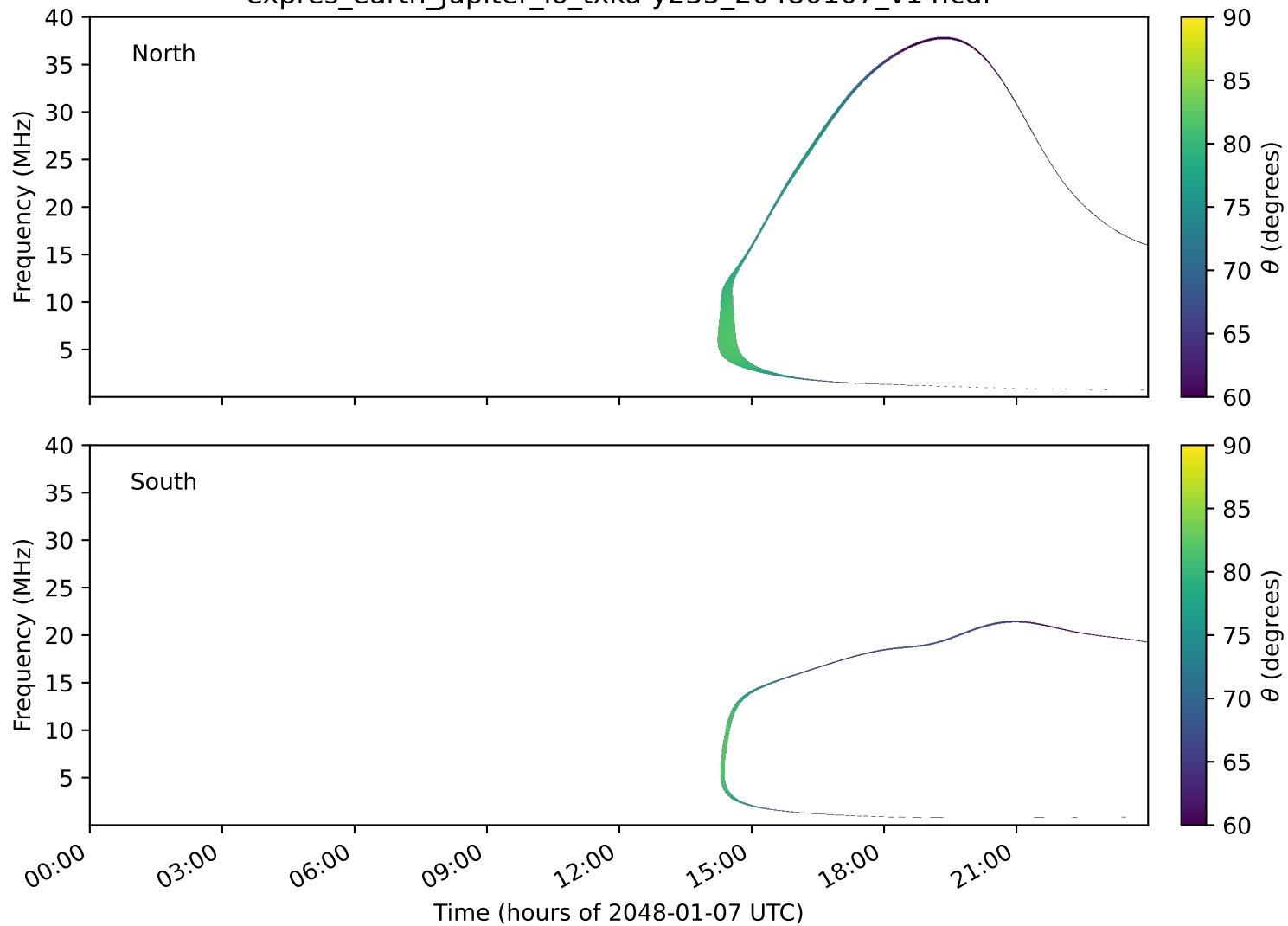
expres_earth_jupiter_io_txka-y235_20480107_v14.cdf
