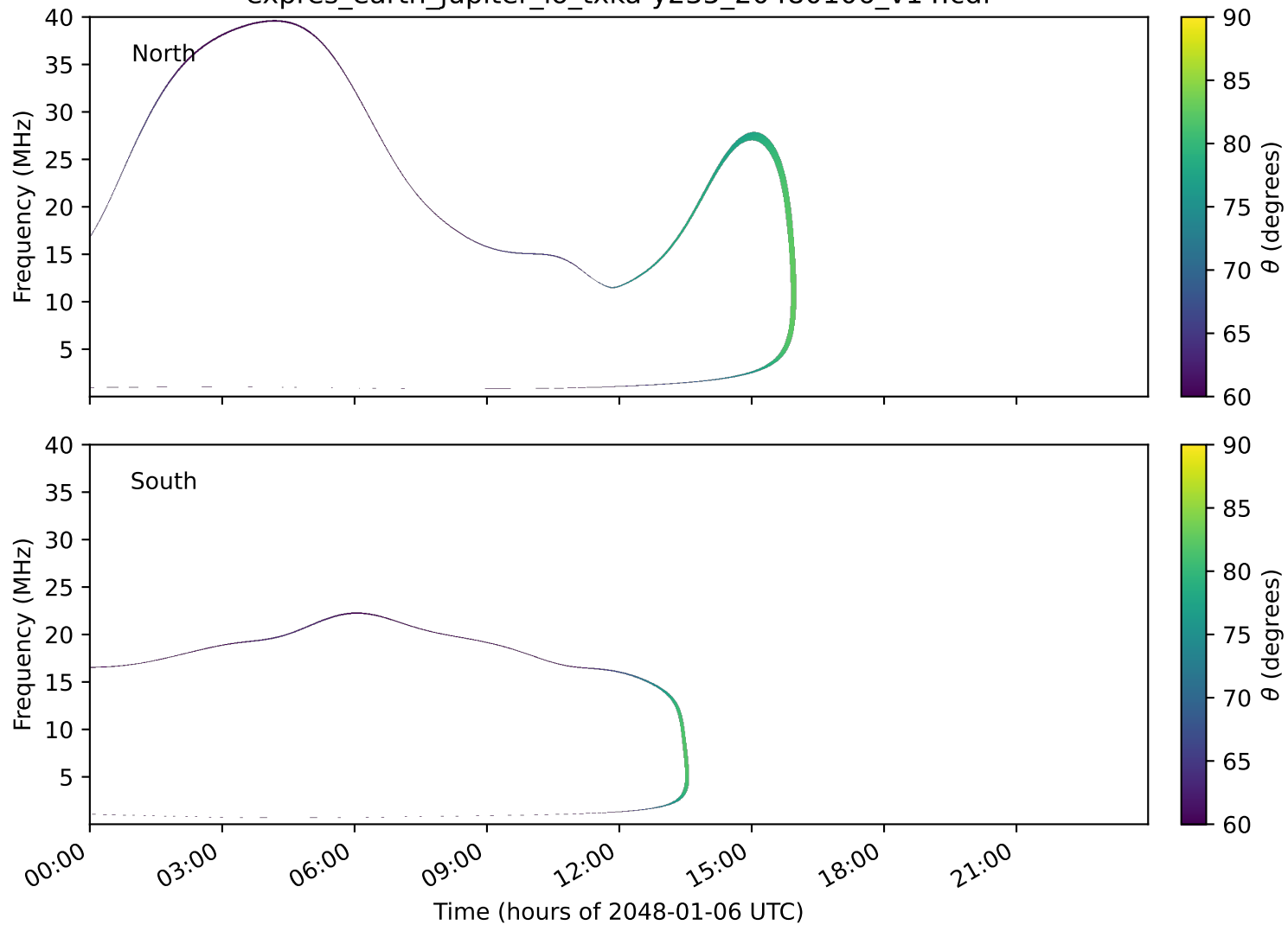
expres_earth_jupiter_io_txka-y235_20480106_v14.cdf
