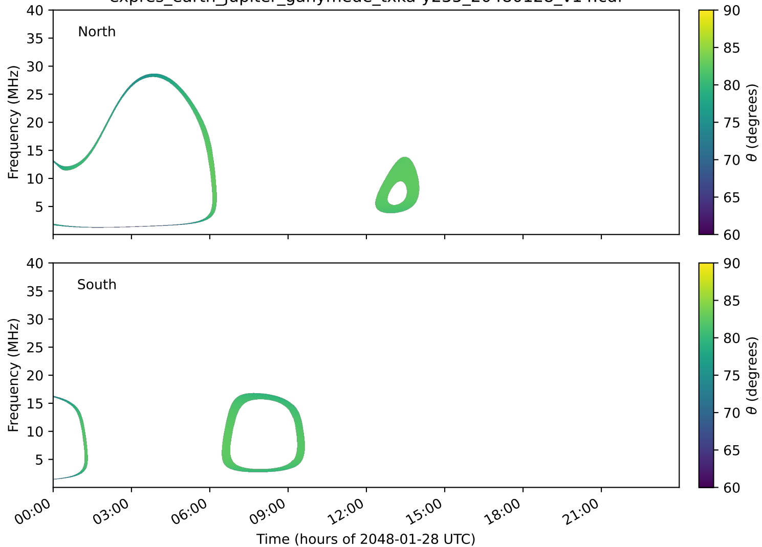
expres_earth_jupiter_ganymede_txka-y235_20480128_v14.cdf
