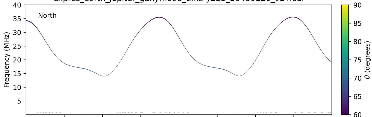
expres_earth_jupiter_ganymede_txka-y235_20480126_v14.cdf
