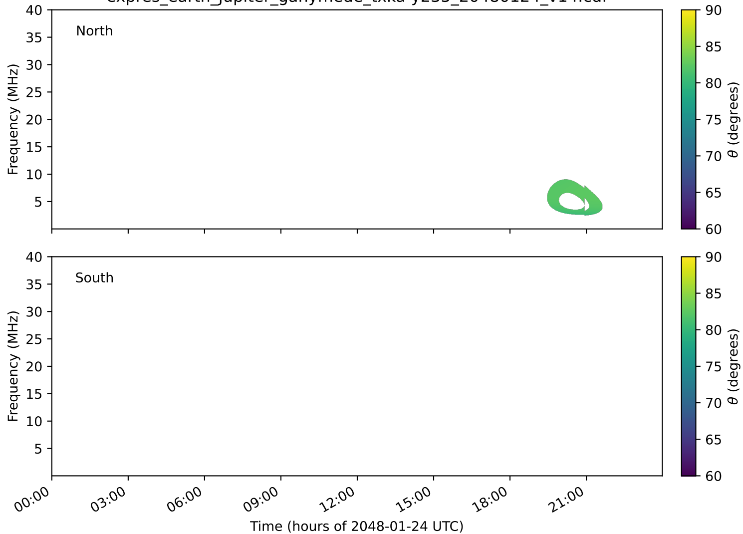
expres_earth_jupiter_ganymede_txka-y235_20480124_v14.cdf
