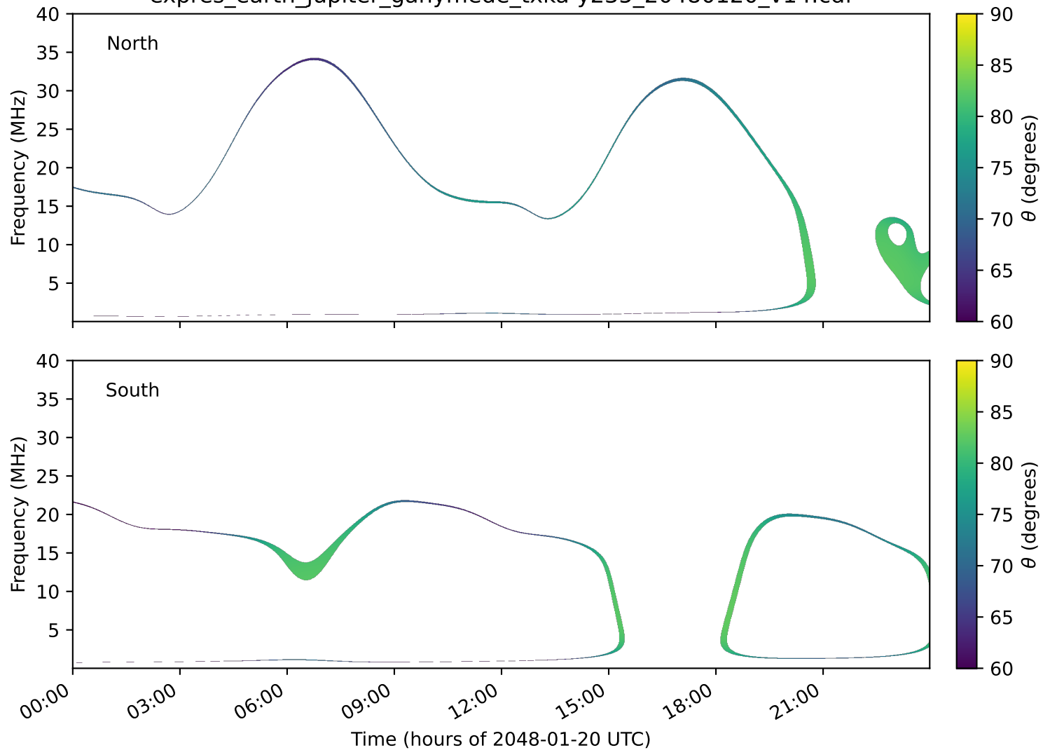
expres_earth_jupiter_ganymede_txka-y235_20480120_v14.cdf
