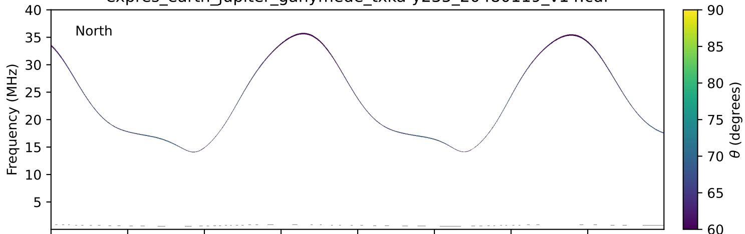
expres_earth_jupiter_ganymede_txka-y235_20480119_v14.cdf
