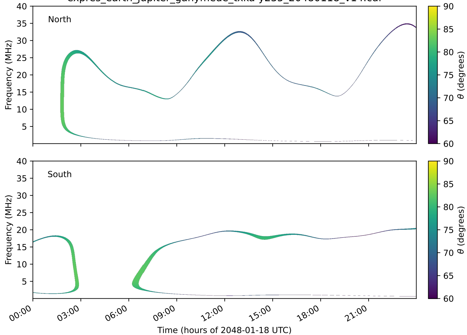
expres_earth_jupiter_ganymede_txka-y235_20480118_v14.cdf
