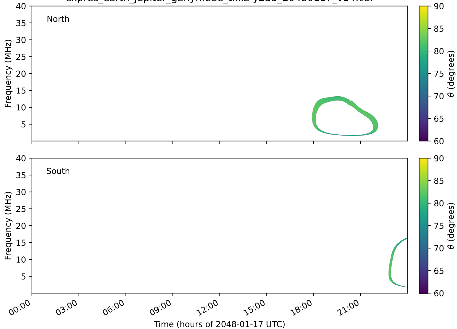
expres_earth_jupiter_ganymede_txka-y235_20480117_v14.cdf
