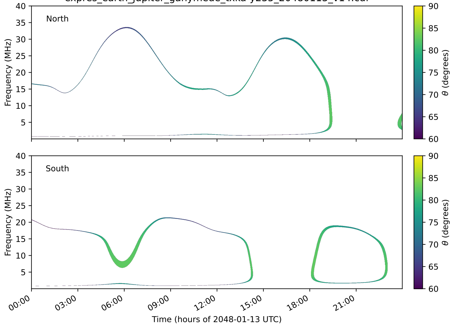
expres_earth_jupiter_ganymede_txka-y235_20480113_v14.cdf
