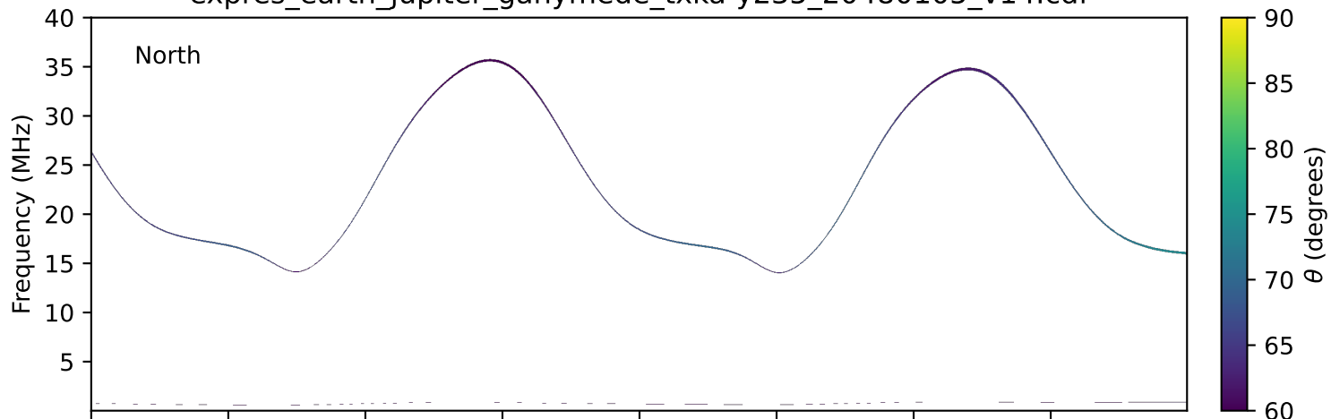
expres_earth_jupiter_ganymede_txka-y235_20480105_v14.cdf
