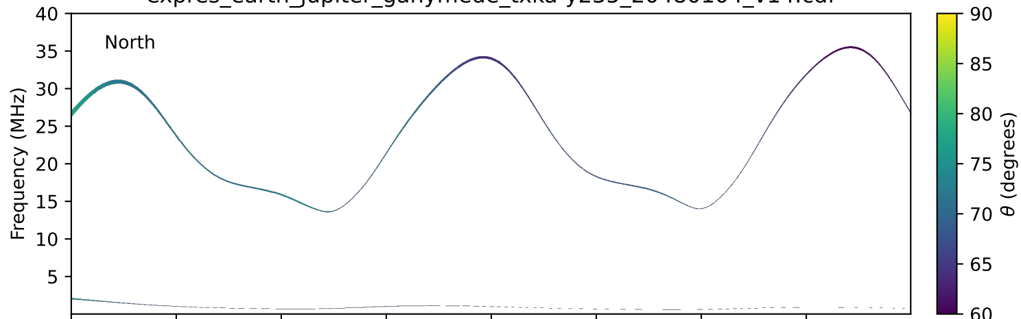
expres_earth_jupiter_ganymede_txka-y235_20480104_v14.cdf
