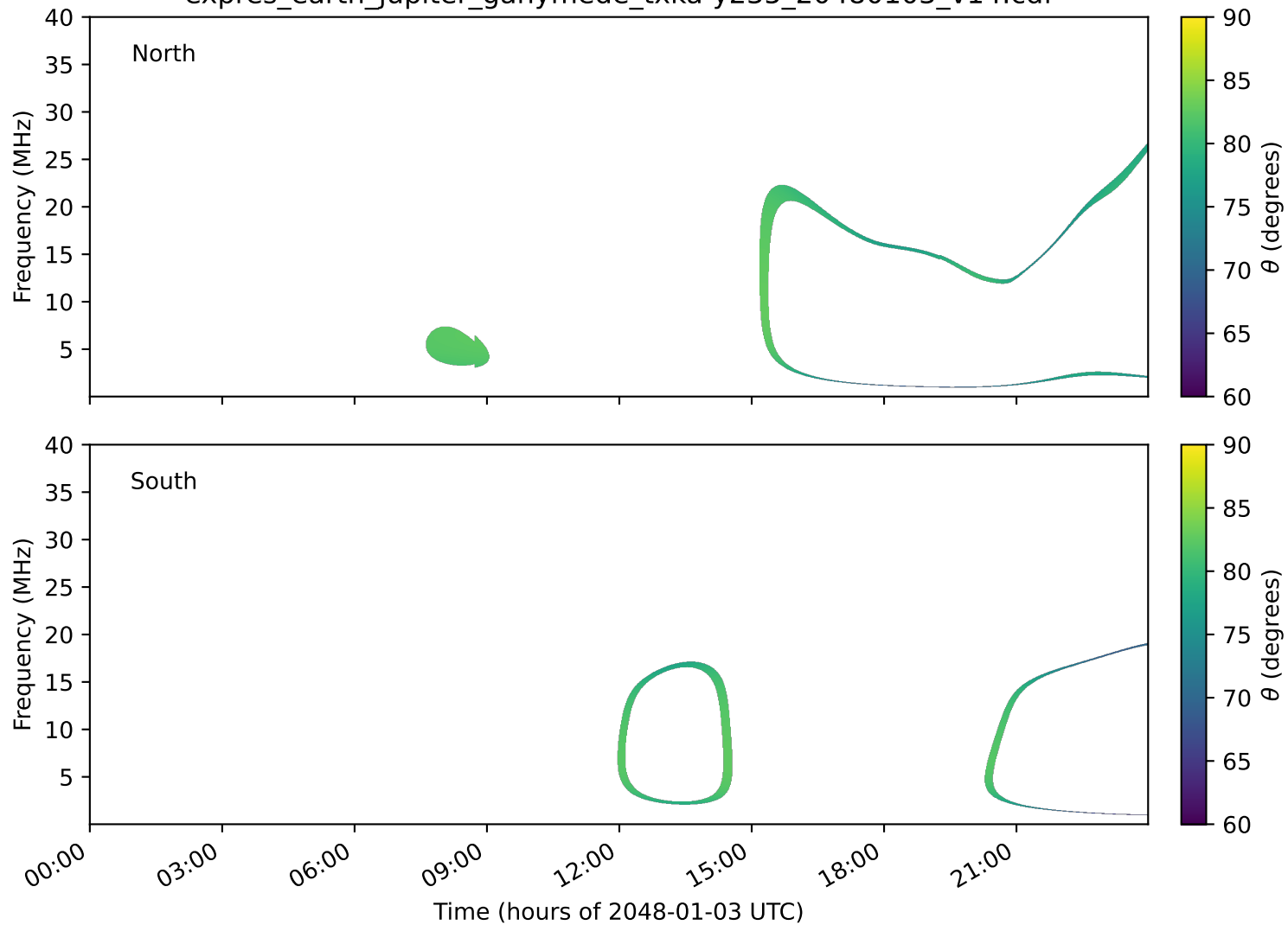
expres_earth_jupiter_ganymede_txka-y235_20480103_v14.cdf
