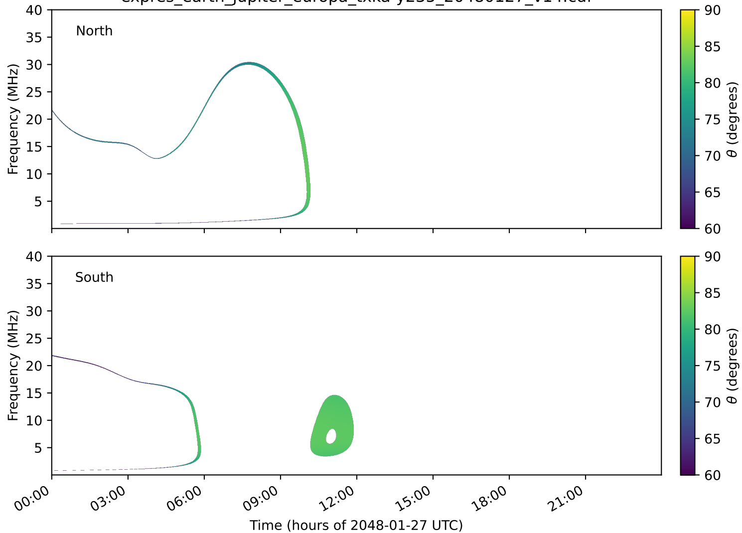
expres_earth_jupiter_europa_txka-y235_20480127_v14.cdf
