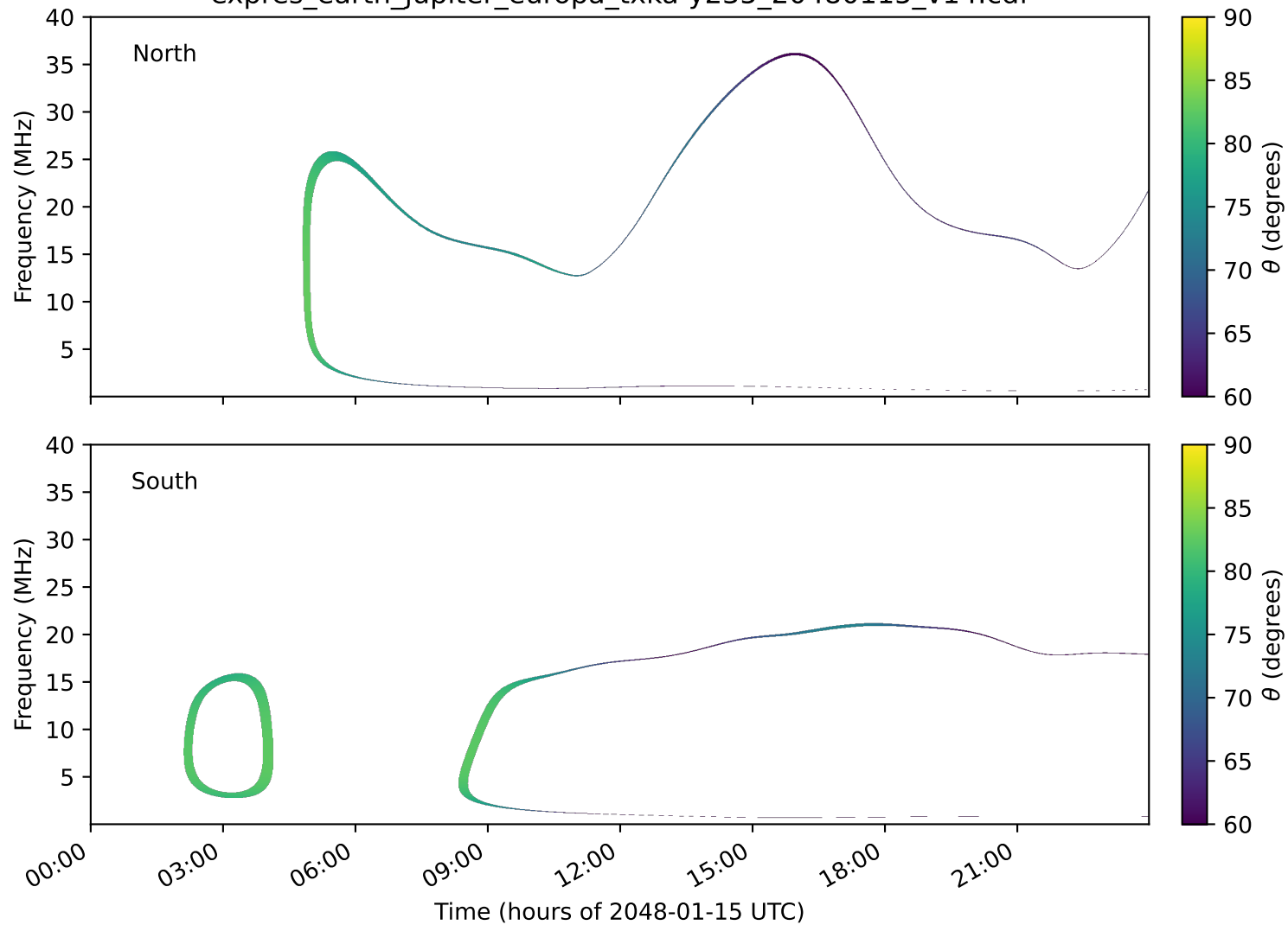
expres_earth_jupiter_europa_txka-y235_20480115_v14.cdf
