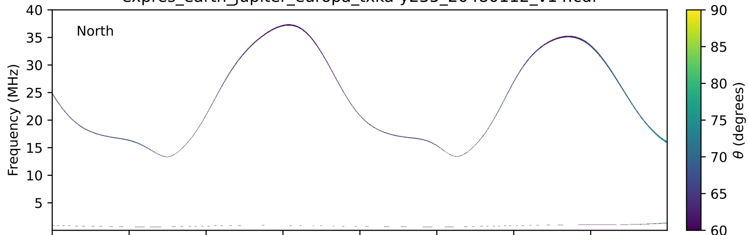
expres_earth_jupiter_europa_txka-y235_20480112_v14.cdf
