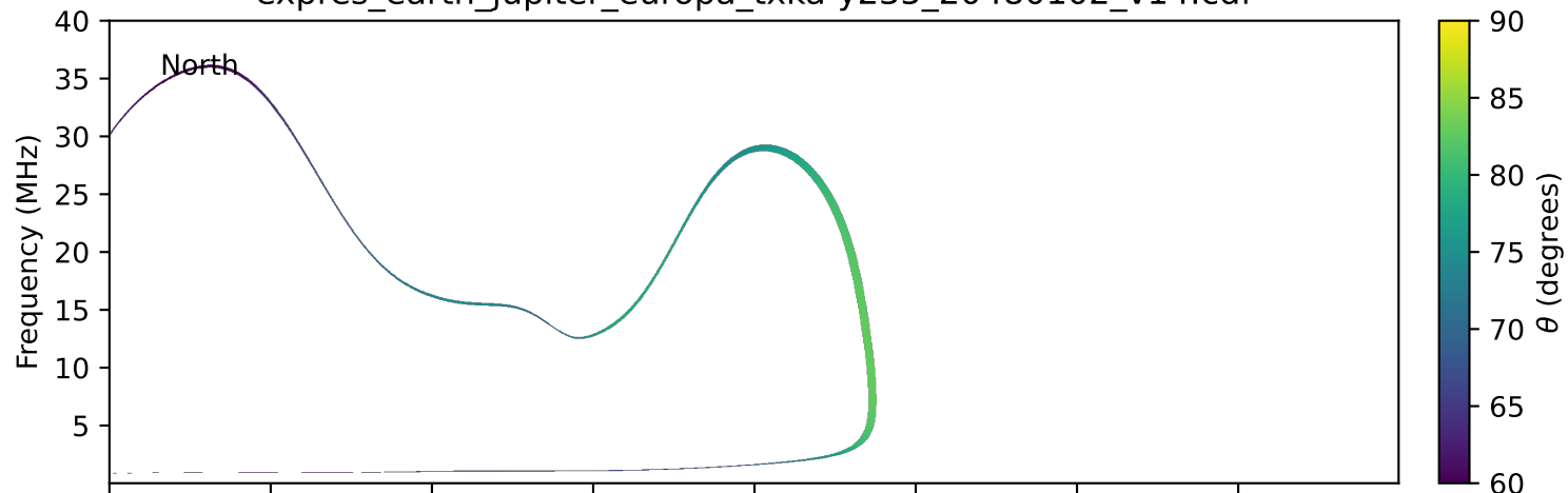
expres_earth_jupiter_europa_txka-y235_20480102_v14.cdf
