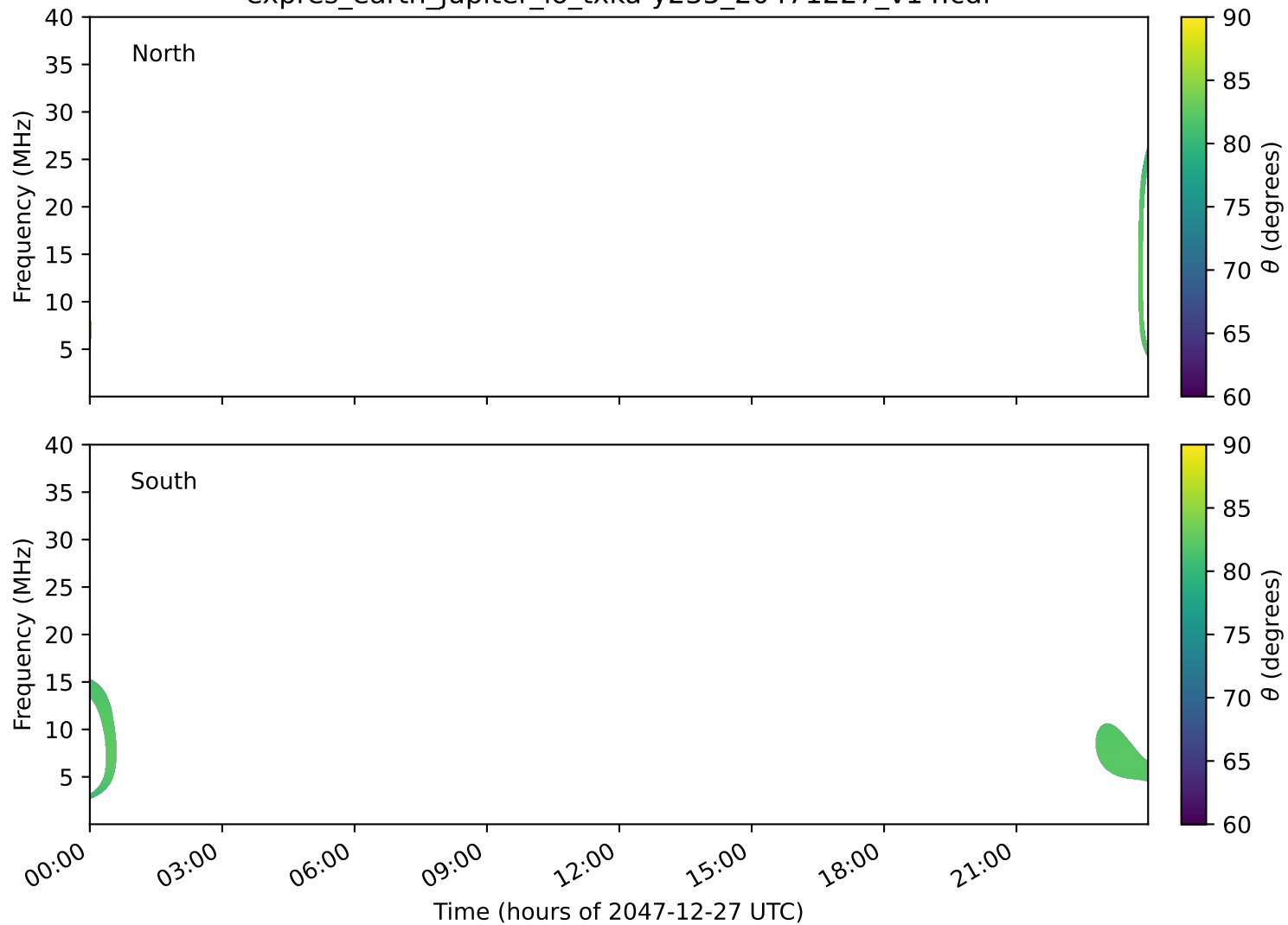
expres_earth_jupiter_io_txka-y235_20471227_v14.cdf
