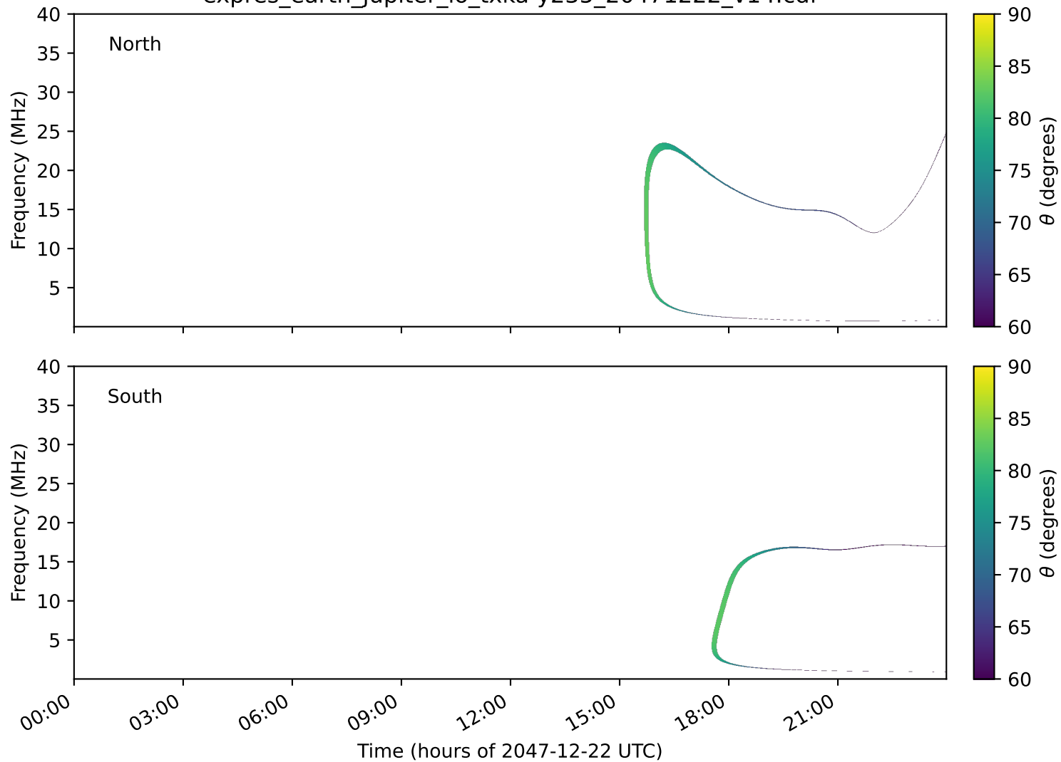
expres_earth_jupiter_io_txka-y235_20471222_v14.cdf
