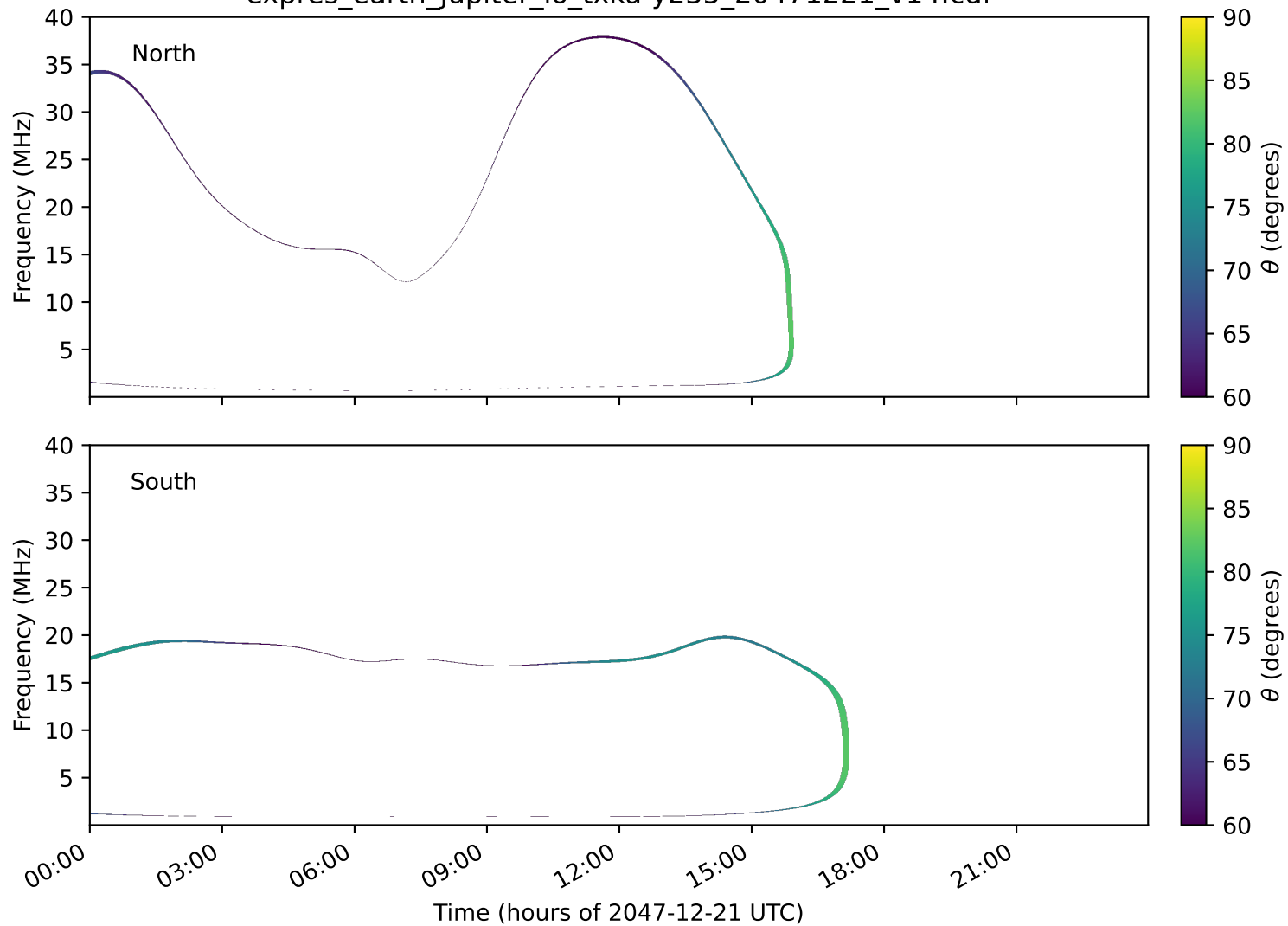
expres_earth_jupiter_io_txka-y235_20471221_v14.cdf
