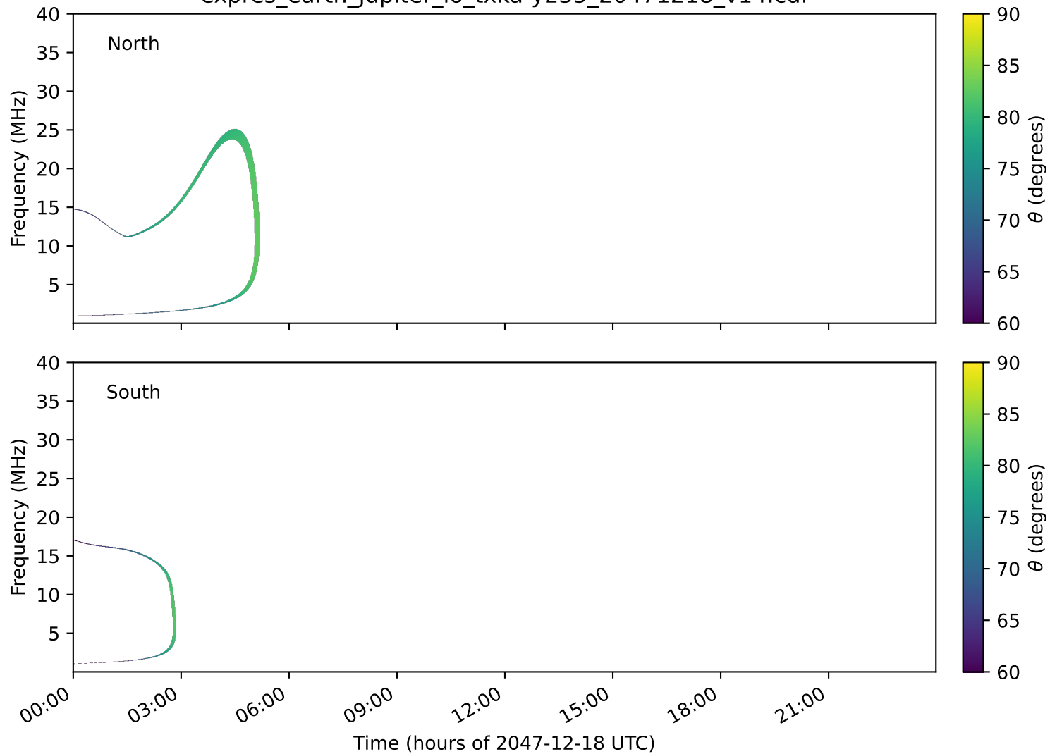
expres_earth_jupiter_io_txka-y235_20471218_v14.cdf
