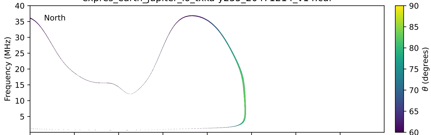
expres_earth_jupiter_io_txka-y235_20471214_v14.cdf
