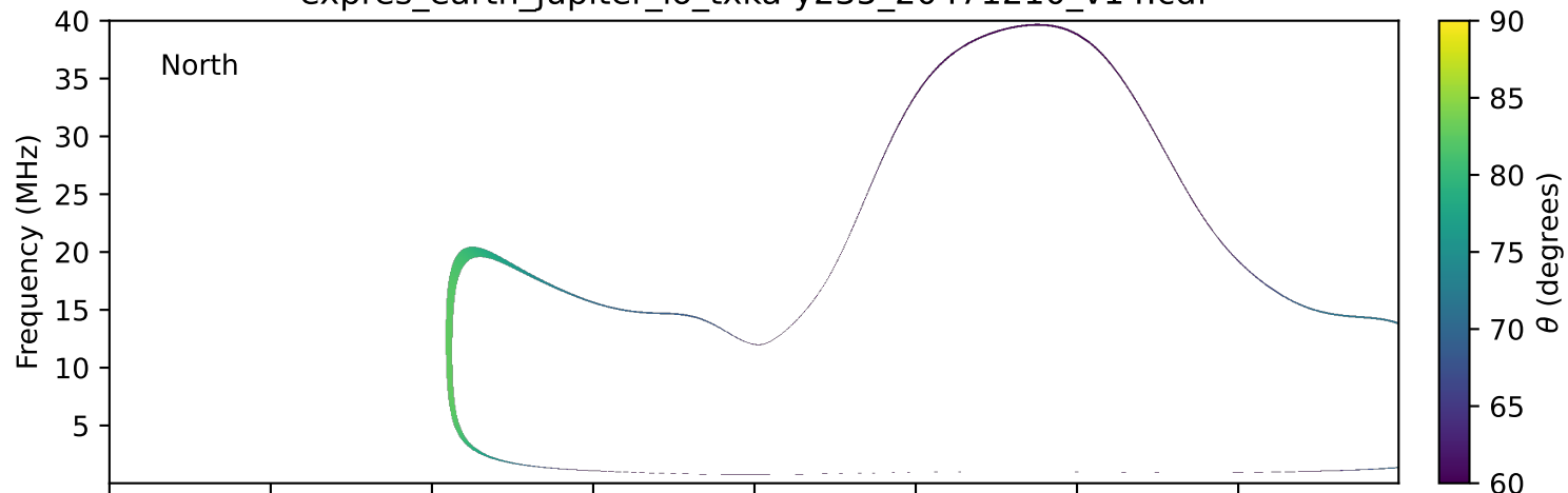
expres_earth_jupiter_io_txka-y235_20471210_v14.cdf
