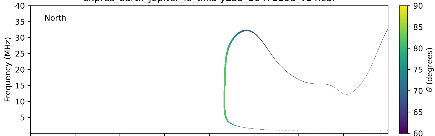
expres_earth_jupiter_io_txka-y235_20471208_v14.cdf
