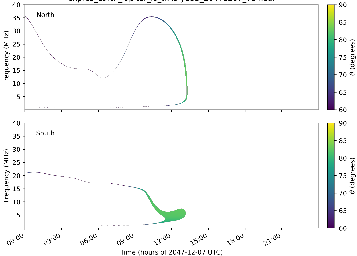
expres_earth_jupiter_io_txka-y235_20471207_v14.cdf
