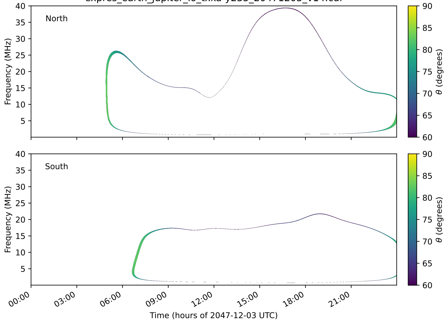
expres_earth_jupiter_io_txka-y235_20471203_v14.cdf
