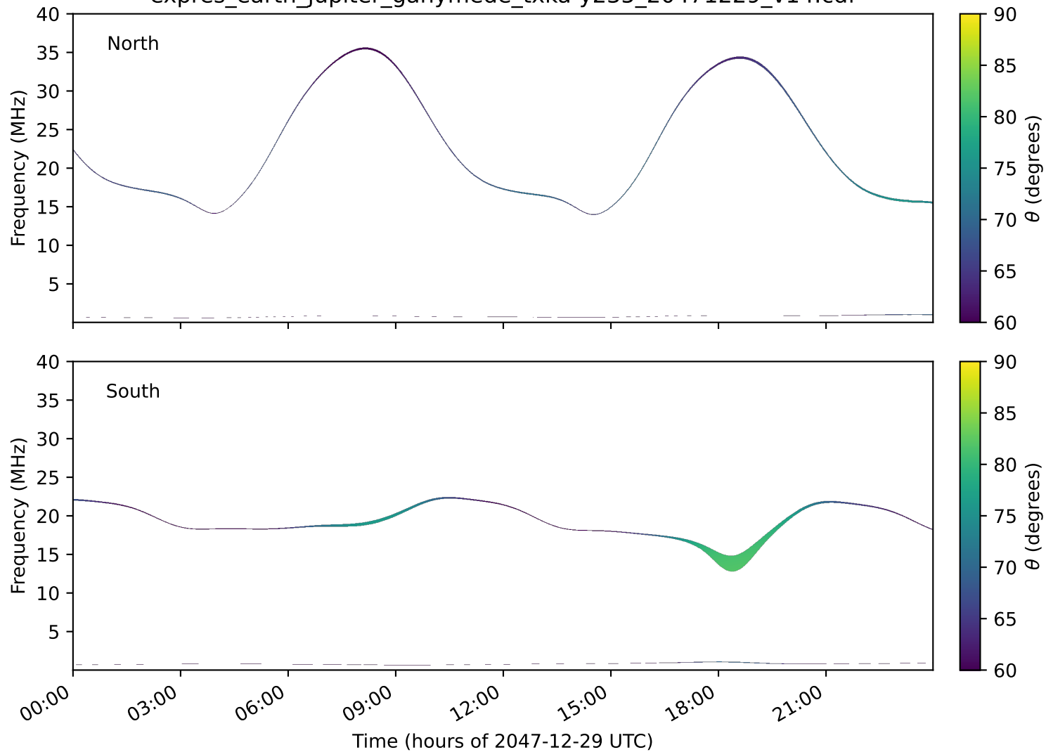
expres_earth_jupiter_ganymede_txka-y235_20471229_v14.cdf
