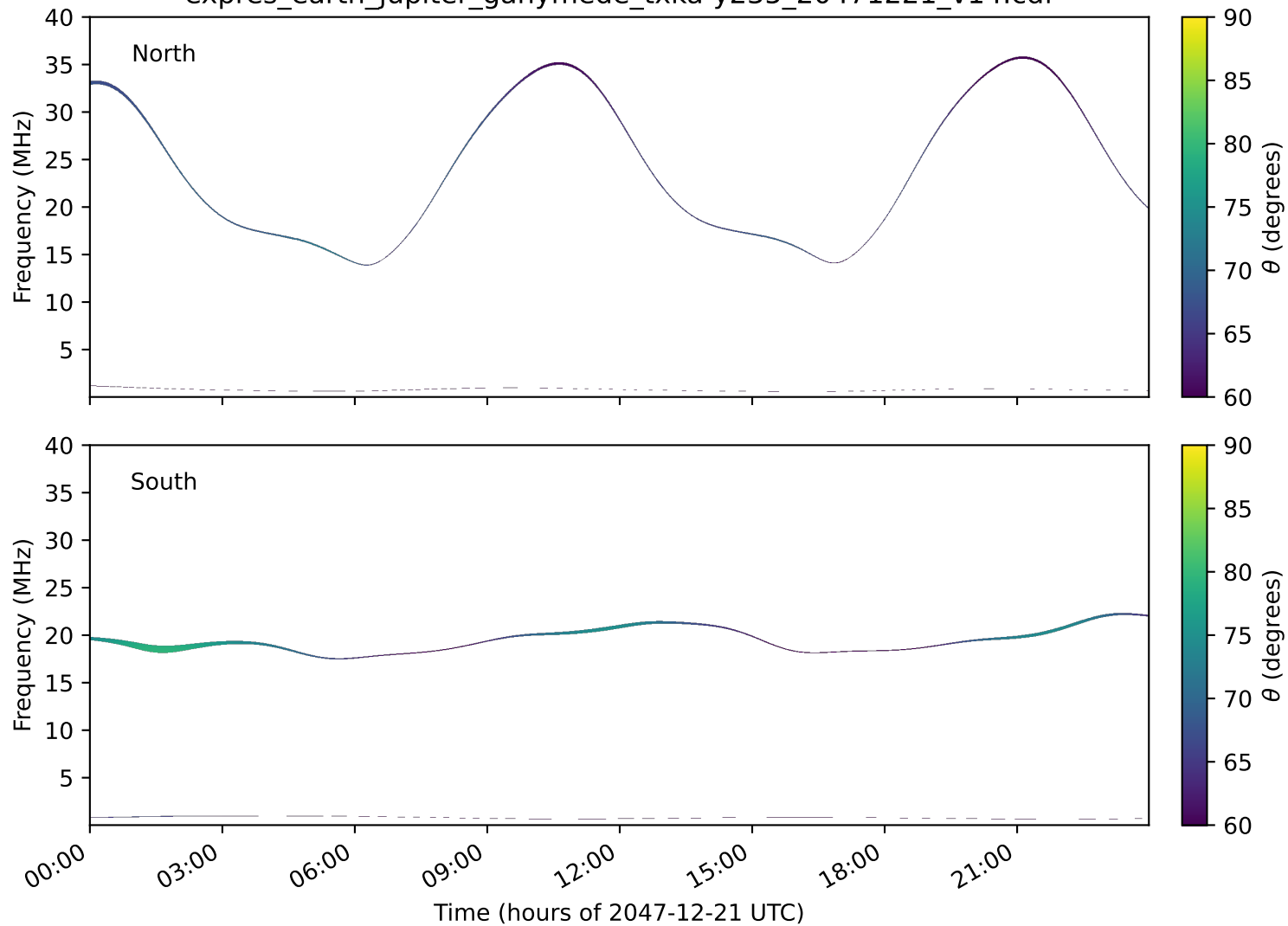
expres_earth_jupiter_ganymede_txka-y235_20471221_v14.cdf
