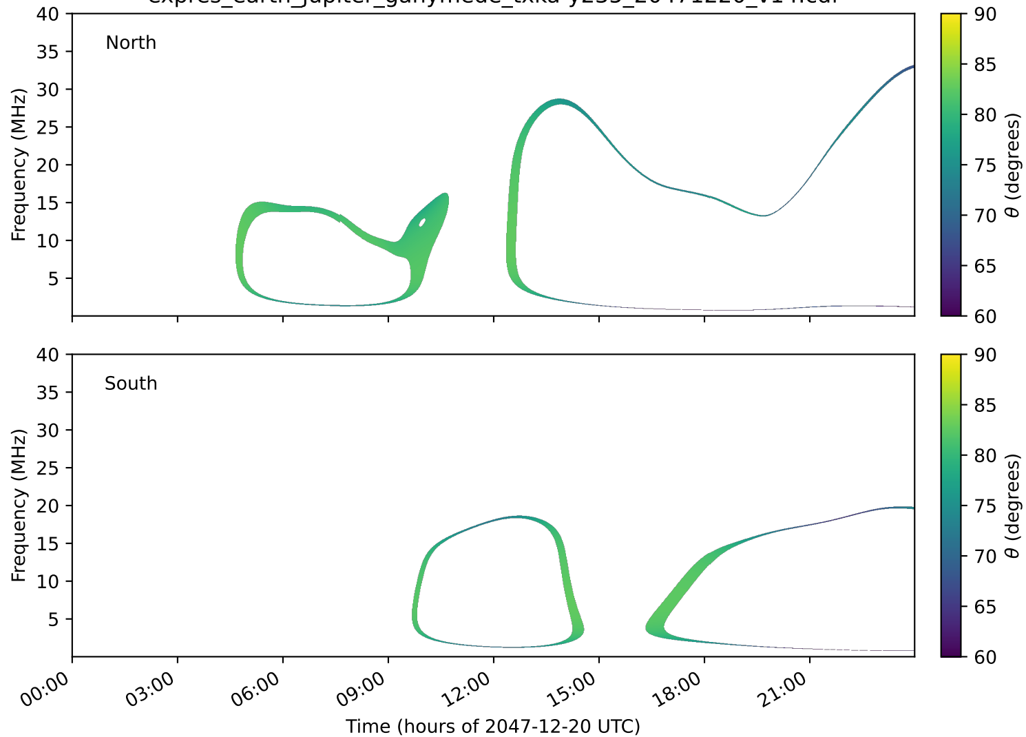
expres_earth_jupiter_ganymede_txka-y235_20471220_v14.cdf
