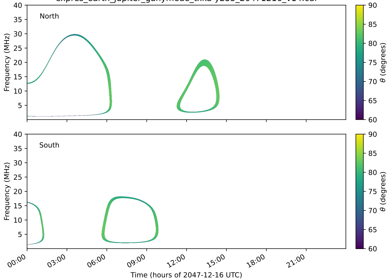
expres_earth_jupiter_ganymede_txka-y235_20471216_v14.cdf
