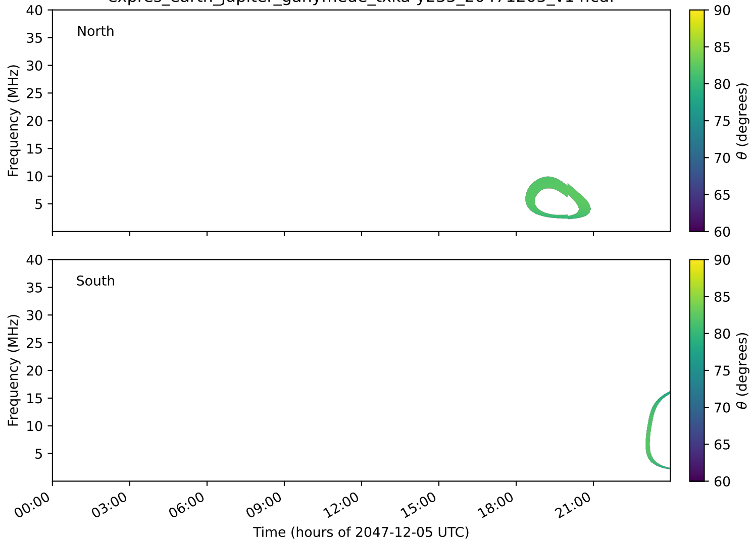
expres_earth_jupiter_ganymede_txka-y235_20471205_v14.cdf
